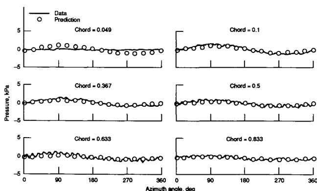
Fig. 12 Azimuthal variation of blade-surface pressure on the pressure surface at r/R = 0.641 , test 6, M = 0.2 , J = 0.881 .
