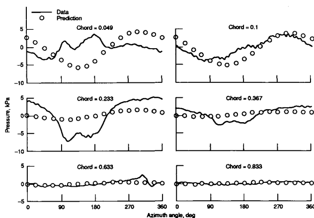
Fig. 13 Azimuthal variation of blade-surface pressure on the suction surface at r/R = 0.641 , test 6, M = 0.2 , J = 0.881 .
