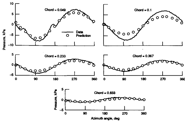
Fig. 7 Azimuthal variation of blade-surface pressure on the suction surface at r/R = 0.641 , test 8, M = 0.5 , J = 3.062 .
