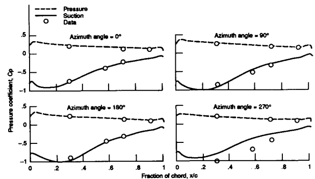
Fig. 10 Predicted and measured azimuthal variation of chordwise pressure coefficient at r/R = 0.9 , test 6, M = 0.2 , J = 0.881 .
