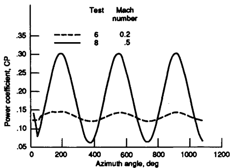
Fig. 4 Power per blade variation with azimuth angle.
