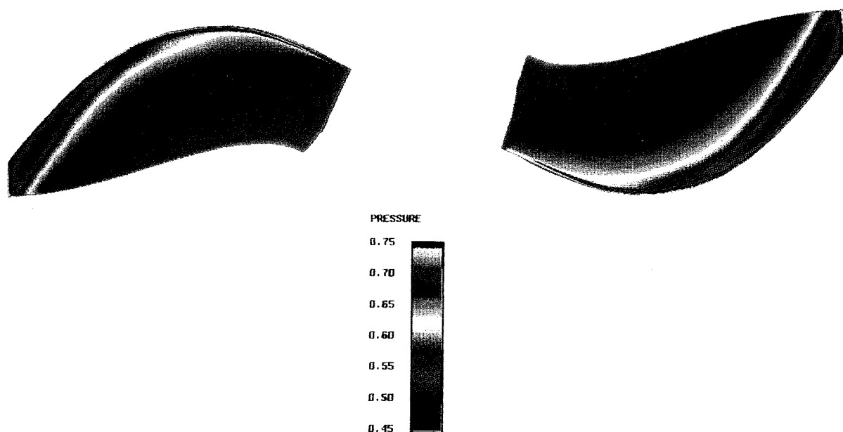
Fig. 11 Static pressure contours on the suction surfaces of the upward moving and downward moving blades: low-pressure region indicates the leading-edge vortex, test 6, M = 0.2 , J = 0.881 , inflow angle = 3 deg.
