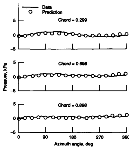
Fig. 14 Azimuthal variation of blade-surface pressure on the pressure surface at r/R = 0.906 , test 6, M = 0.2 , J = 0.881 .
