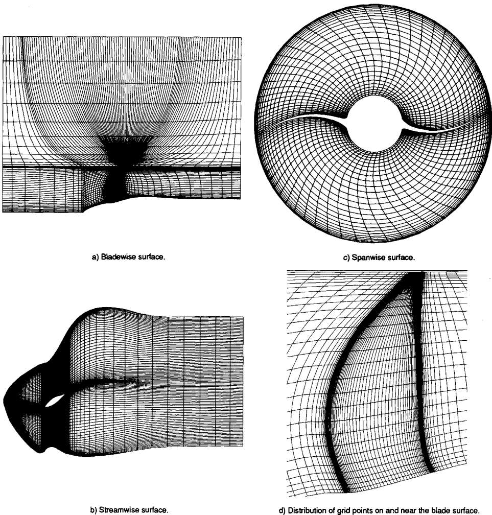
Fig. 3 Typical computational grid.
