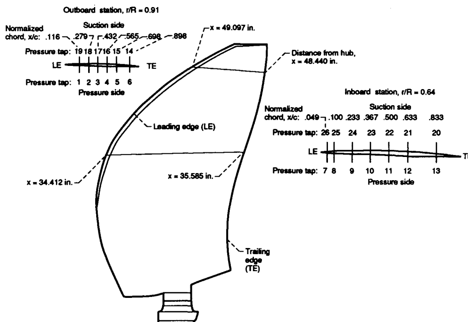
Fig. 1 Transducer locations for unsteady pressure measurements.
