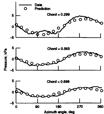
Fig. 9 Azimuthal variation of blade-surface pressure on the suction surface at r/R = 0.906 , test 8, M = 0.5 , J = 3.062 .
