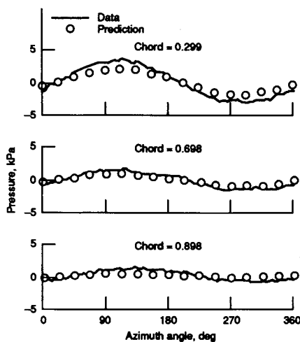
Fig. 8 Azimuthal variation of blade-surface pressure on the pressure surface at r/R = 0.906 , test 8, M = 0.5 , J = 3.062 .
