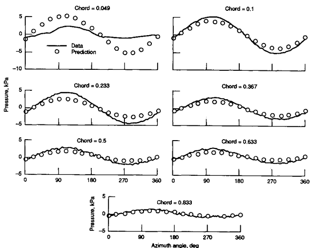
Fig. 6 Azimuthal variation of blade-surface pressure on the pressure surface at r/R = 0.641 , test 8, M = 0.5 , J = 3.062 .
