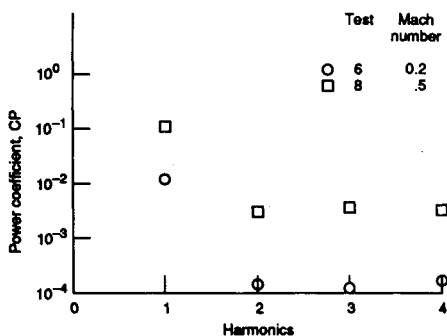
Fig. 5 Loading spectrum.
