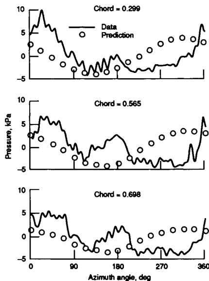
Fig. 15 Azimuthal variation of blade surface pressure on the suction surface at r/R = 0.906 , test 6, M = 0.2 , J = 0.881 .
